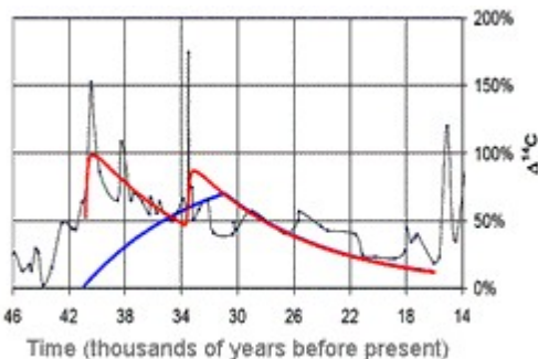
Radiocarbon peaks in Icelandic marine sediment samples, indicated by the black line, coincide with three supernova-caused events that Firestone and Wells believe led to the extinction of the mammoth.
